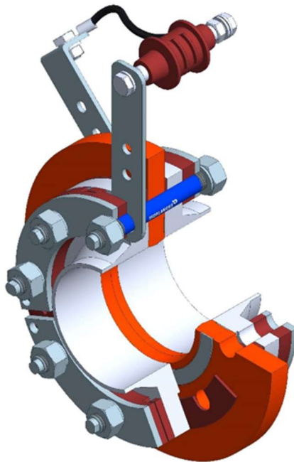
Figure 1: Example of installation with cable lug and spark gap
