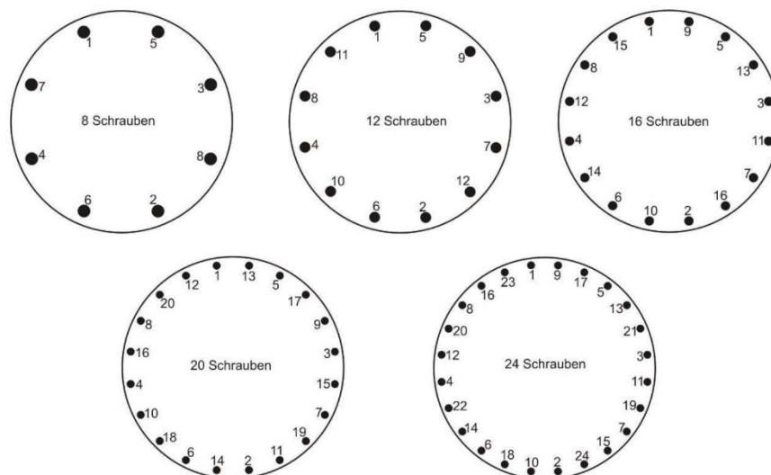
Figure 2: Tightening sequence of the bolts
