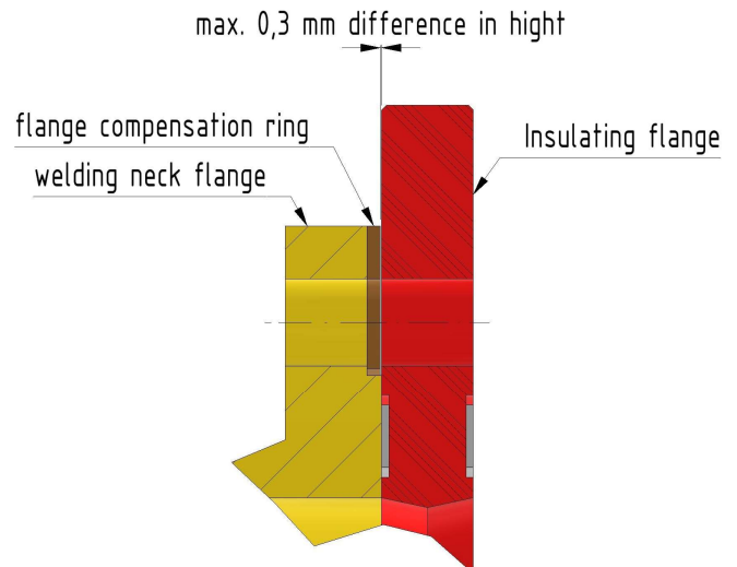
Figure 7: Flange compensation ring assembly
